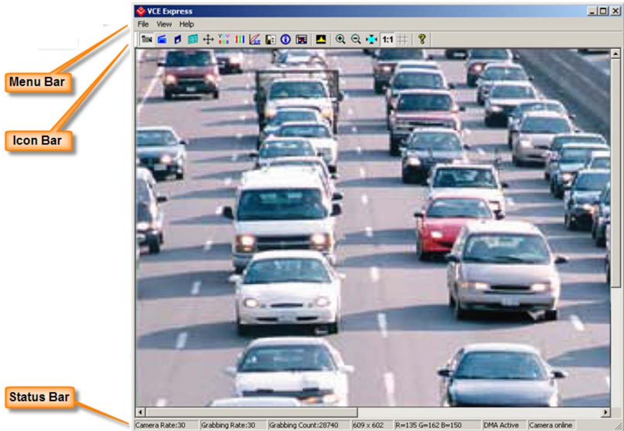
Figure 3 – Main dialog
