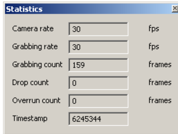
Figure 14 – Statistics dialog
